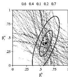
Figure 6.3 A Tomography Plot. Each coordinate represents a unique value of \beta_i^b and \beta_i^w . Each line traces out, for a particular combination of T_i and X_i , the algebraic expression in Equation 6.27. The contour lines on the figure represent the truncated bivariate normal distribution of \beta_i^b and \beta_i^w , with parameters \hat{\mu}_i^b , \hat{\mu}_i^w , \hat{\sigma}_i^b , \hat{\sigma}_i^w and \hat{\rho} indicated at the top of the graph. (See Figure 6.4 for a surface plot representation of these contours, which may be more familiar.)
