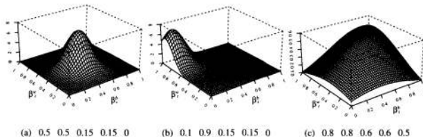
Figure 6.2 Truncated Bivariate Normal Distributions, TN(\beta_i^b, \beta_i^w | \tilde{\Sigma}, \tilde{\mu}) . Graph (a) is a distribution relatively unaffected by the truncation bounds. The graphs (b) and (c) are strongly truncated. Parameter values \tilde{\mu} , \tilde{\Sigma} , \tilde{\sigma}_b , \tilde{\sigma}_w , and \tilde{\rho} are indicated beneath each graph.
