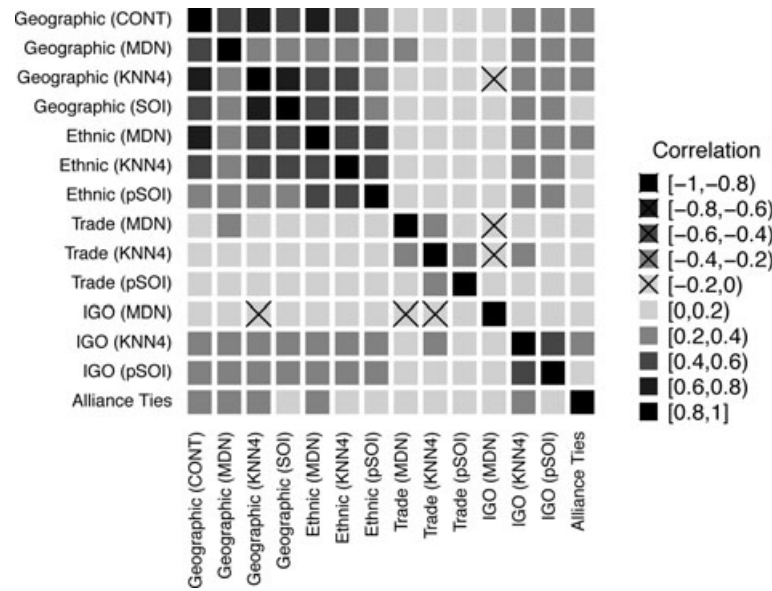
FIG 4. Structural similarity. Shadings correspond to size and direction of graph correlation statistics for every pair of network specifications shown in Figure 3.
