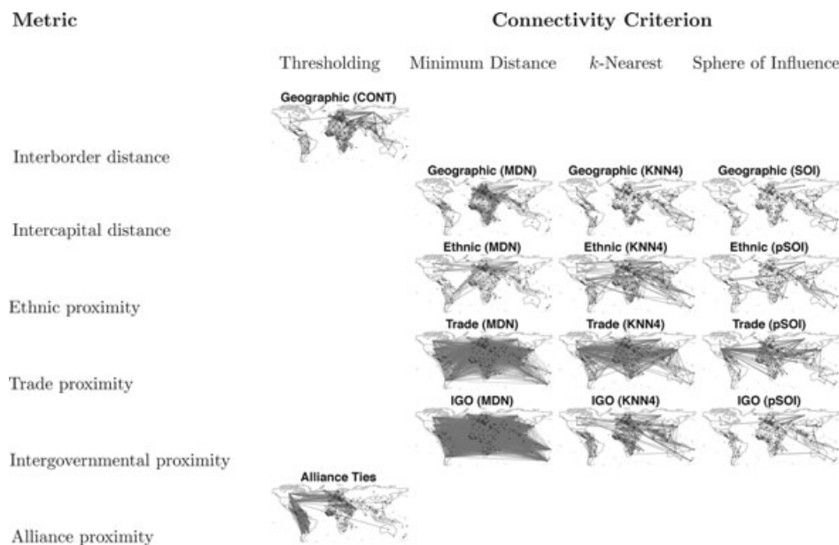
FIG 3. Network specifications. Gray lines indicate the existence of a connection between each pair of country according to each distance or proximity metric and connectivity criterion.
