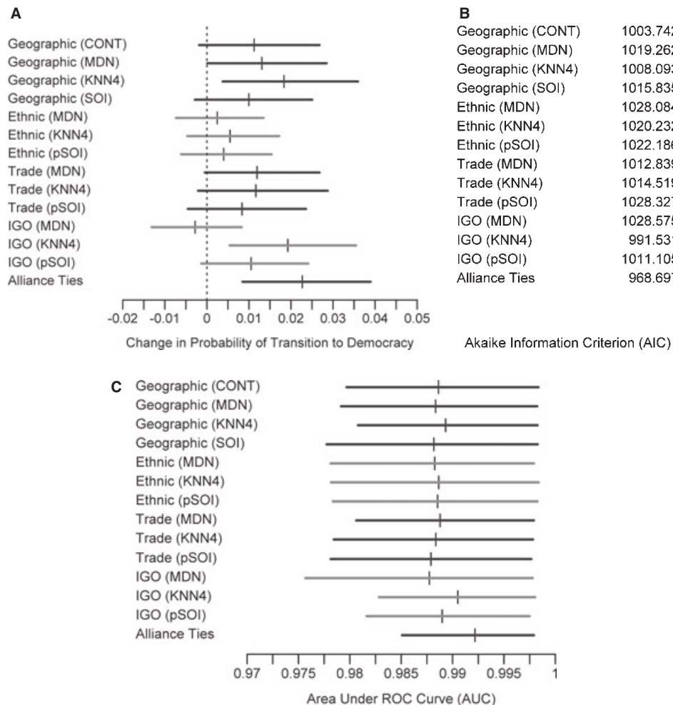
FIG 5. Model fit diagnostics. (a) Strength of autocorrelation. (b) Goodness-of-fit. (c) Cross-validation. Figures show [5a] changes in transition probability due to a single standard deviation increase above the mean in the proportion of neighboring democracies, holding all other variables at their means, [5b] model AIC statistics, and [5c] out-of-sample areas under the ROC curve, averaged over 100 random data partitions.
