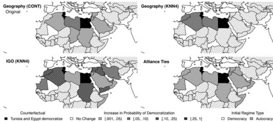
FIG 6. Arab Spring simulation. Average change in transition probability after 1,000 simulations.
