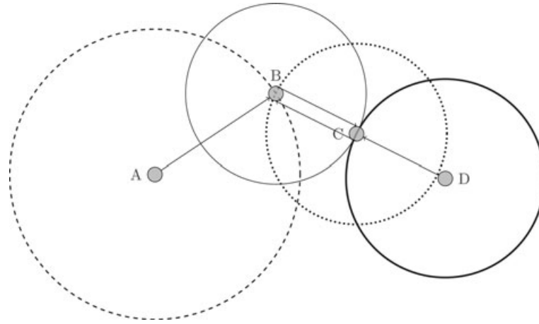
FIG 2. Sphere of influence graph. Nodes represent cities, and directed edges (radii of circles) correspond to nearest neighbor distances. Here, city B is the nearest neighbor of city A , B and C are nearest neighbors of each other, and C is the nearest neighbor of D . Where the circles around reach city overlap in at least two points, the cities can be considered neighbors. In the current example, A is a neighbor of B and C but not D , B is a neighbor of A and C , C is a neighbor to all, and D is a neighbor only of C .
