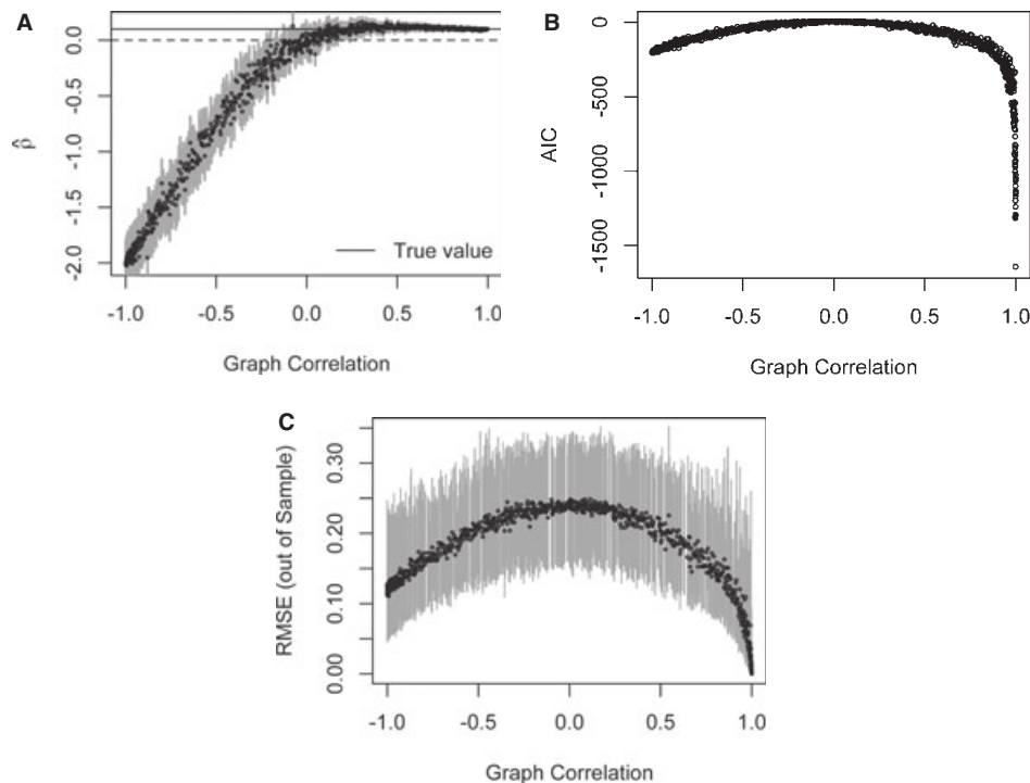
FIG 1. Structural similarity and model selection. Plots show results of Monte Carlo simulation with 1,000 random graphs. Horizontal axes in each plot display the graph correlation of each graph C_m with the true matrix C . The vertical axes report statistics corresponding to [1a] spatial autocorrelation parameter estimates, [1b] AIC statistics, and [1c] out-of-sample RMSE means. (a) Strength of autocorrelation. (b) Goodness-of-fit. (c) Cross-validation.
